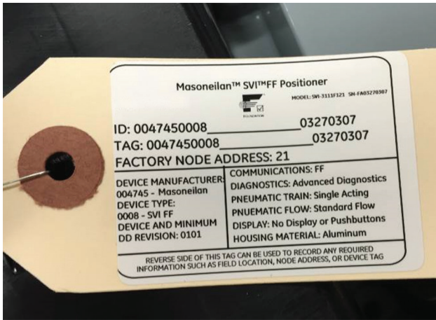
Figure 1 - Unit Tag
