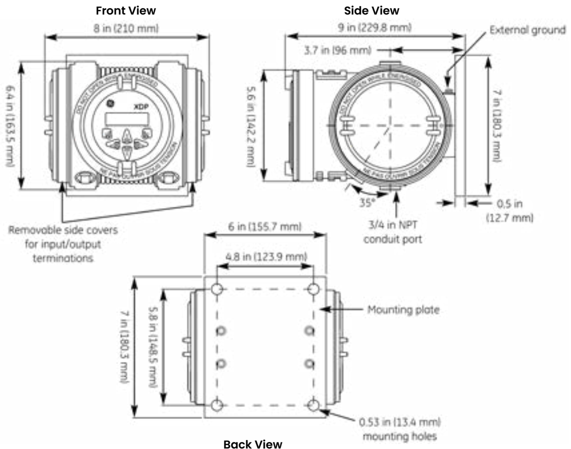
XDP dimensions in inches (mm)
